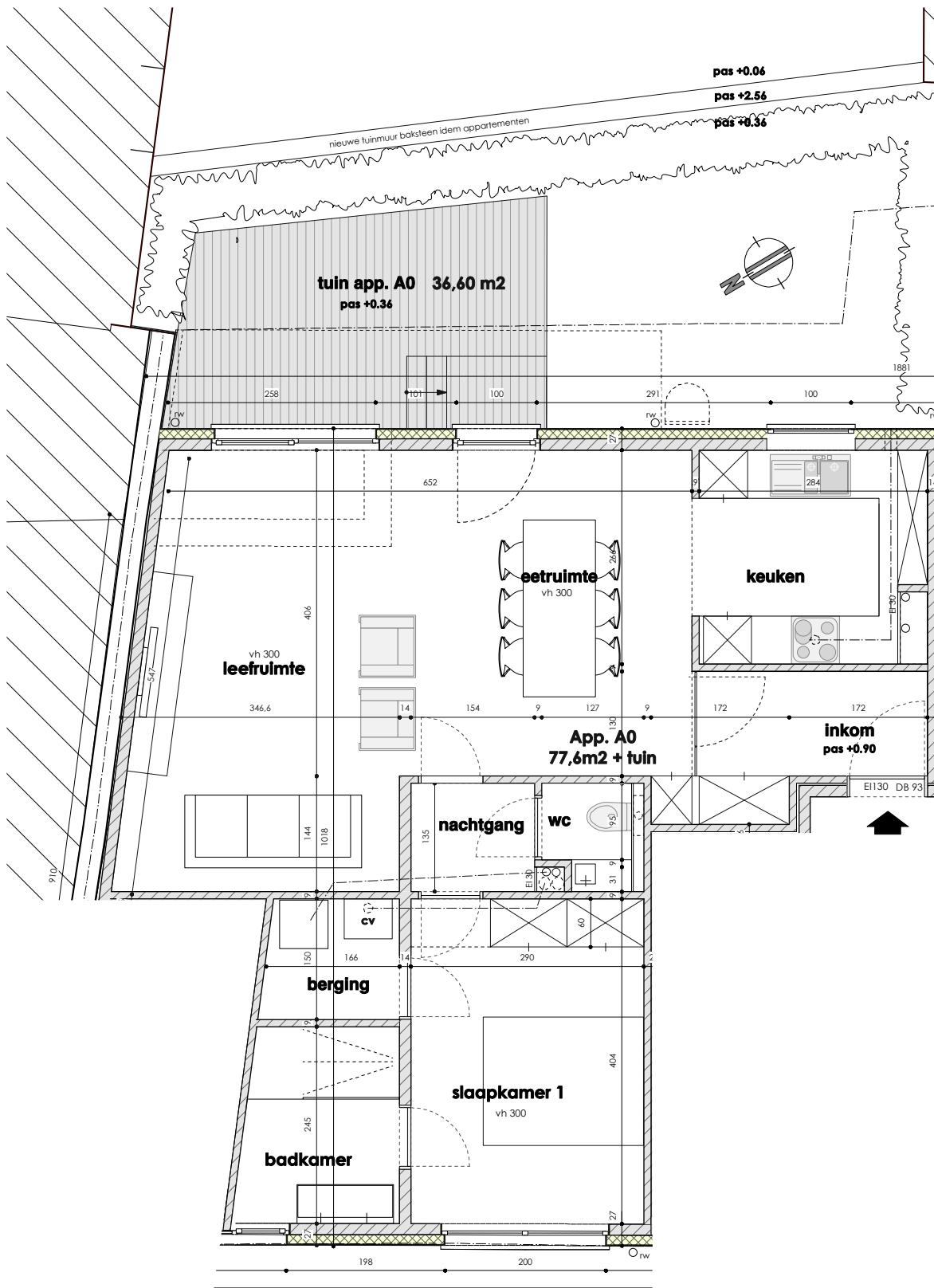
GRONDPLAN A0 1/75
